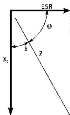
FIGURE 7a Total Impedance of the Capacitor Below Resonance
