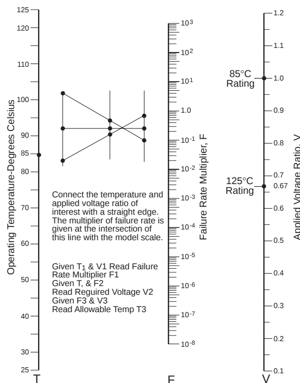
FIGURE 11 Reliability Nomograph
