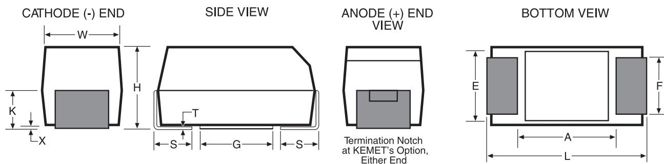
Outline Drawing
