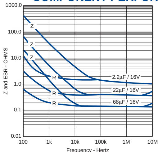
FIGURE 9b ESR &amp; Impedance (Z) vs Frequency
