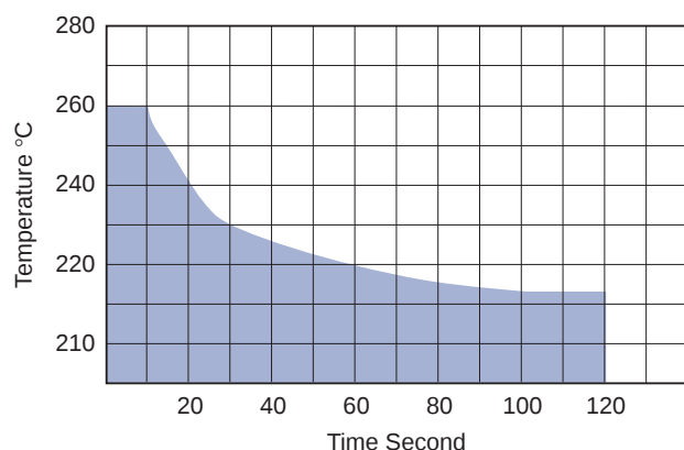
FIGURE 13 Time/Temperature Soldering Profile
