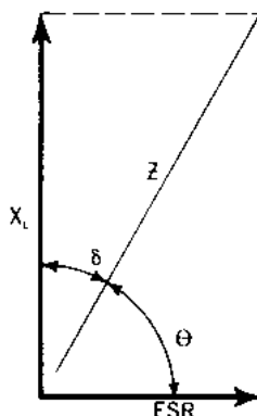
FIGURE 7b Total Impedance of the Capacitor Above Resonance
